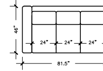
SOFA B W: 81.5" D: 46" H:30" ARM H: 23" SEAT D: 28"
