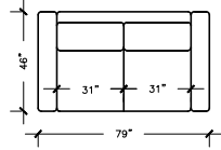
APARTMENT SOFA W: 79" D: 46" H:30" ARM H: 23" SEAT D: 28"
