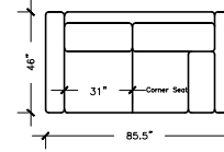
APARTMENT SOFA D W: 85.5" D: 46" H:30" ARM H: 23" SEAT D: 28"
