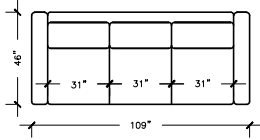
SOFA PLUS W: 109" D: 46" H:30" ARM H: 23" SEAT D: 28"
