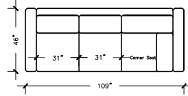
SOFA PLUS D W: 109" D: 46" H:30" ARM H: 23" SEAT D: 28"
